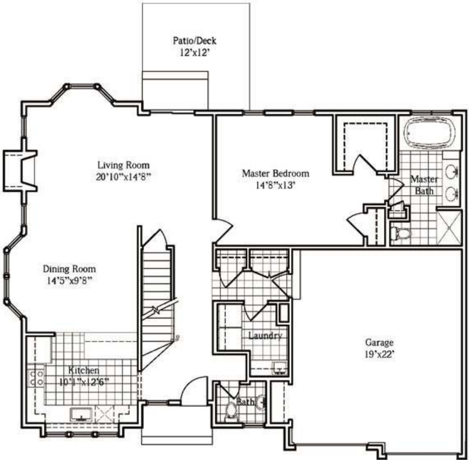
ASHMONT FIRST FLOOR PLAN DEERFIELD ESTATES HOPKINTON, MASSACHUSETTS
